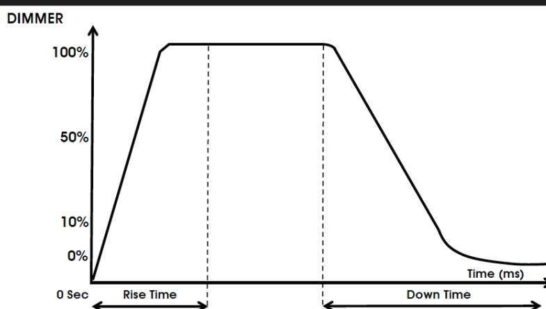
Dimmer Curve Chart
