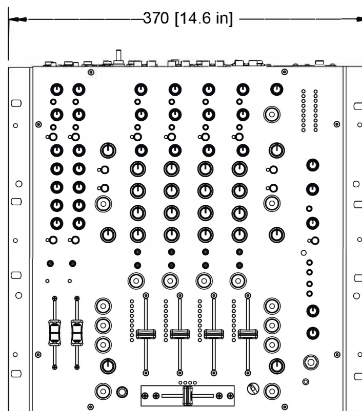
Xone:92 MkII Dimensions with optional Rack Ear Kit fitted [A&H PART NUMBER: X:922-RK19/X]
