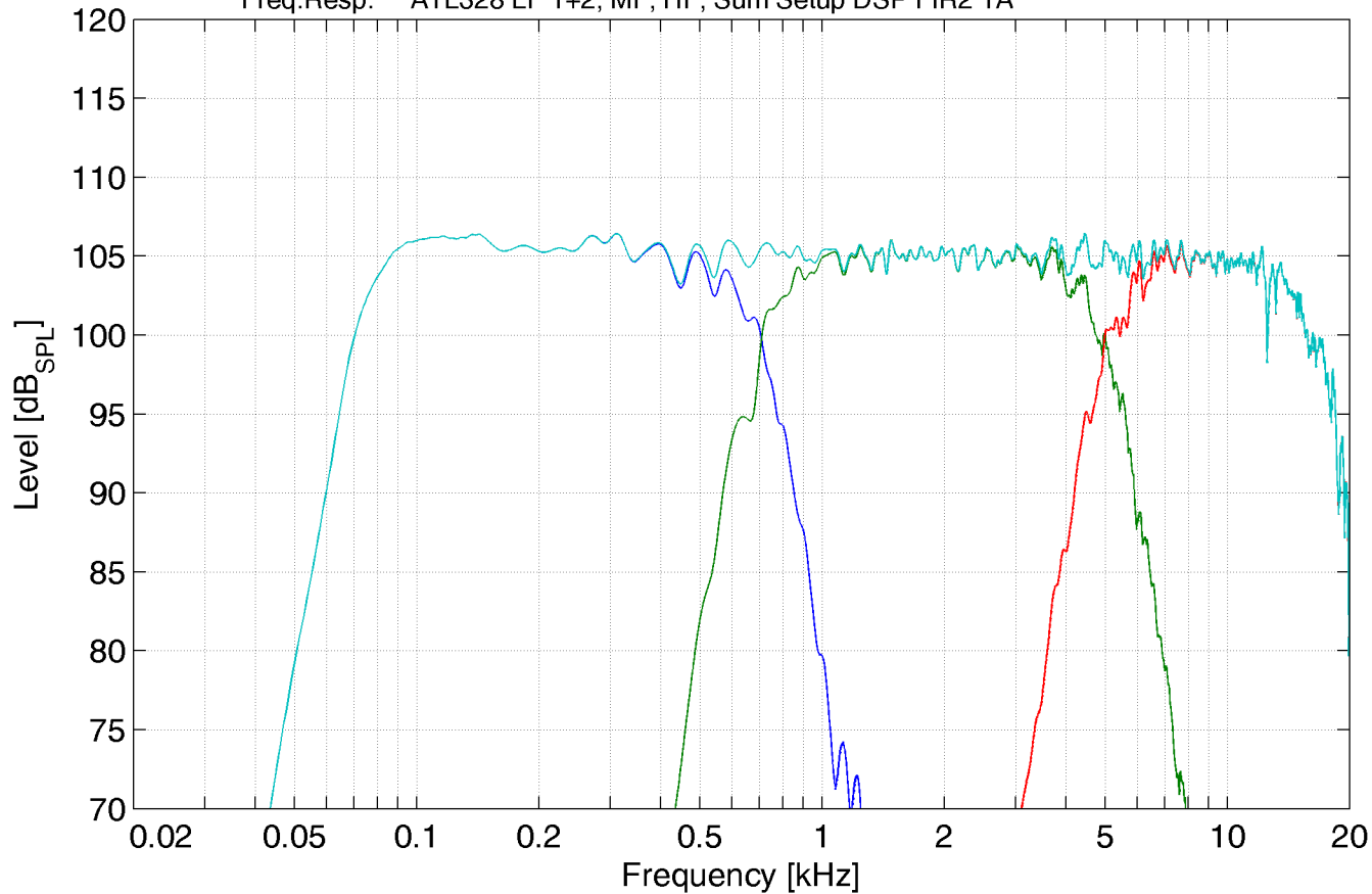
Freq.Resp. ATL328 LF 1+2, MF, HF, Sum Setup DSP FIR2 1A
