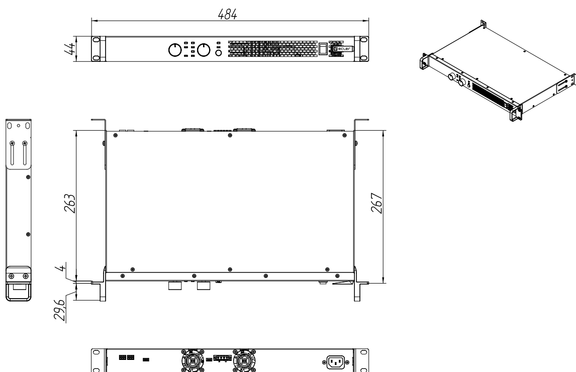
Ecler AURA-2B300 Mechanical Diagram
