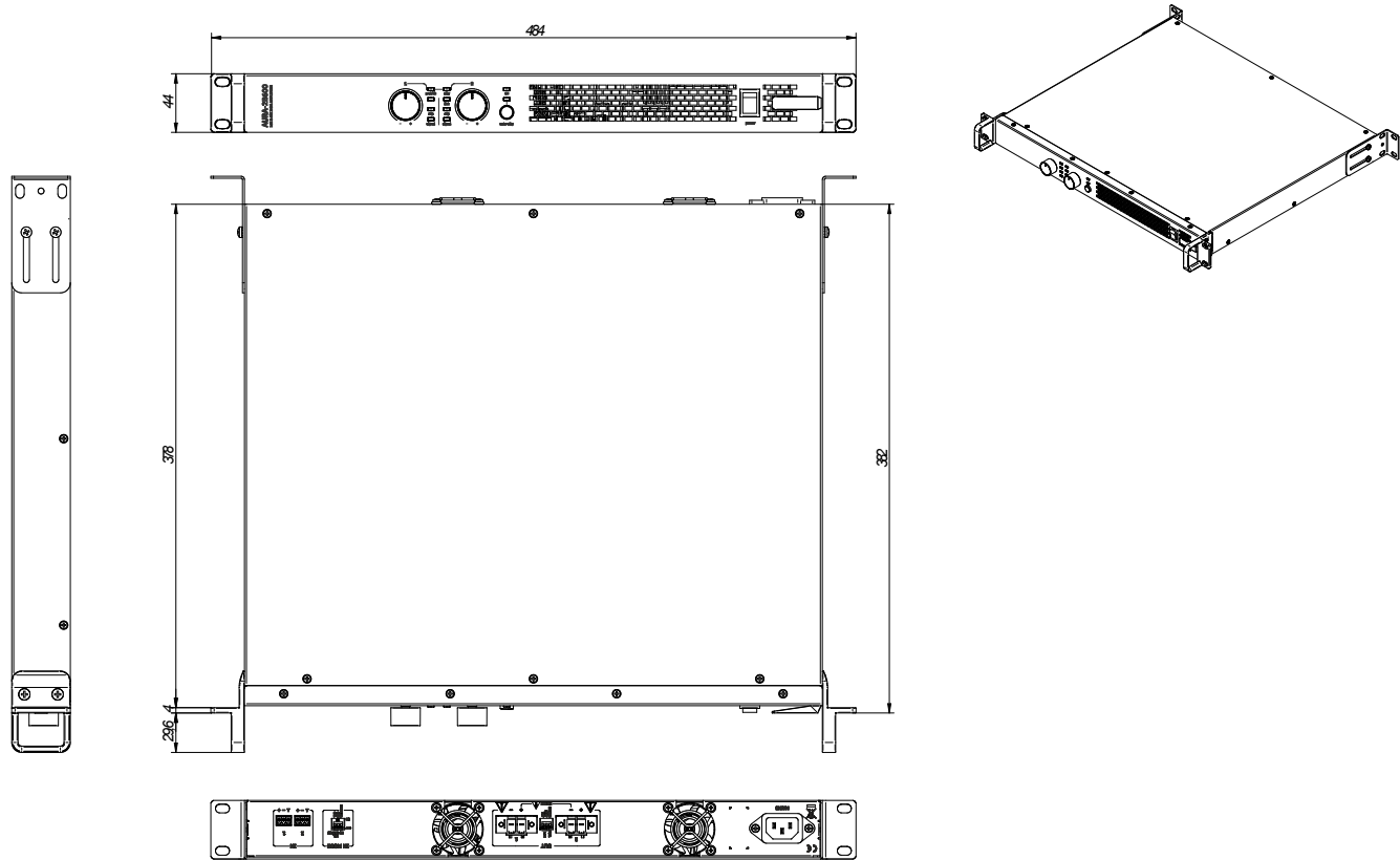
Ecler AURA-2B600 Mechanical Diagram
