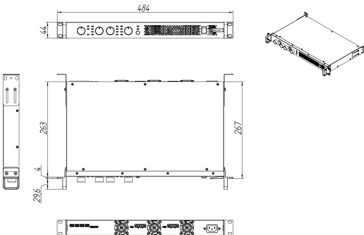
Ecler AURA-4B300 Mechanical Diagram
